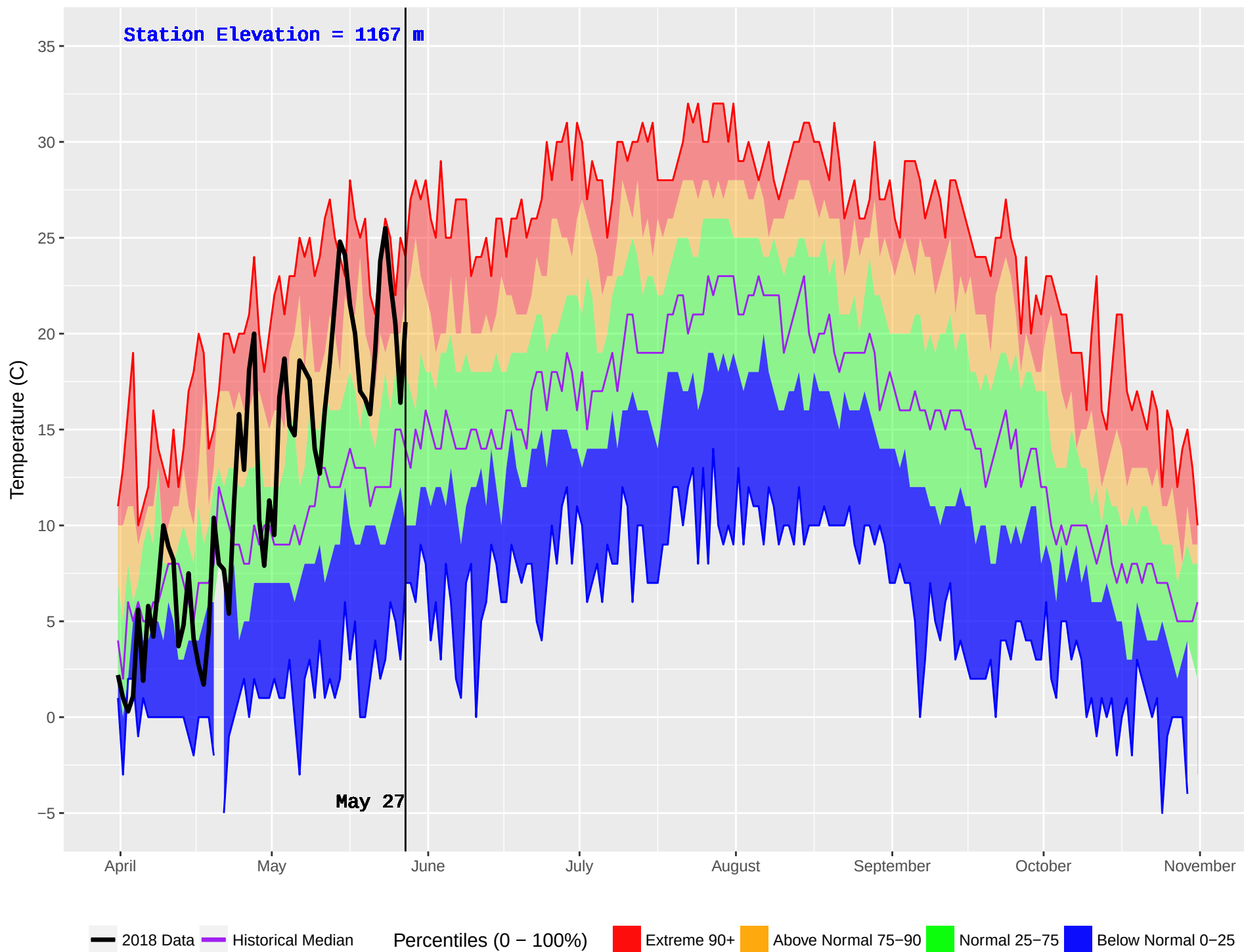
LEIGHTON LAKE (307) : Historical (1982–2016) and Current (2018) Noon Temperature
