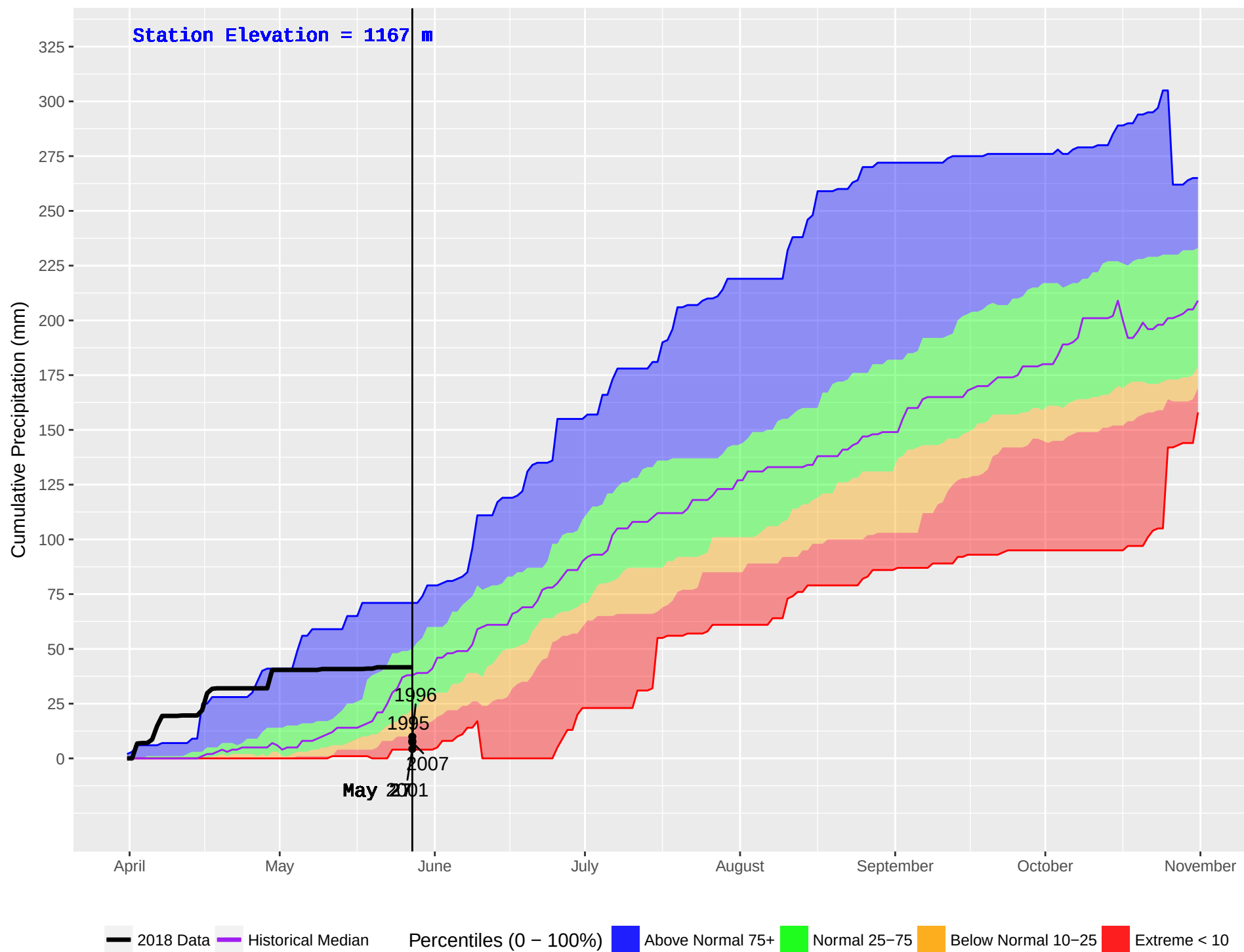
LEIGHTON LAKE (307) : Historical (1982–2016) and Current (2018) Noon Cumulative Precipitation
