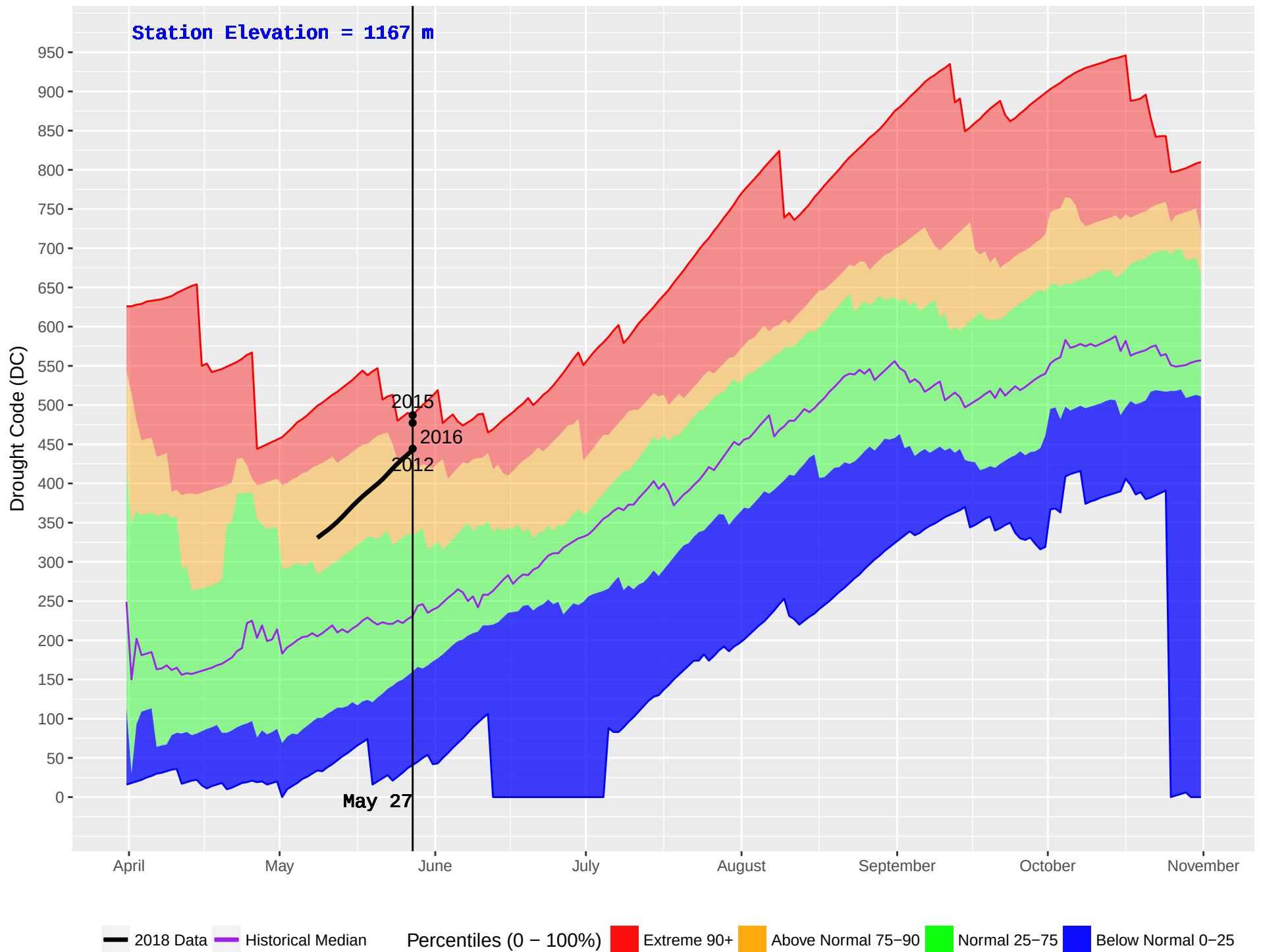
LEIGHTON LAKE (307) : Historical (1982–2016) and Current (2018) Noon Drought Code (DC)
